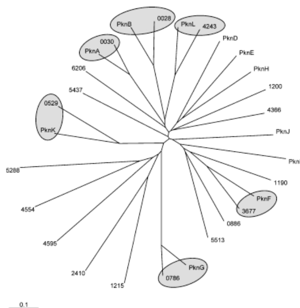
Fig. 1. Dendrogram of a multiple sequence alignment of all the STPKs from Mycobacterium tuberculosis and Mycobacterium smegmatis . Sequences of M. tuberculosis (designated as Pkn's) and M. smegmatis (designated by locus number) kinases obtained from the Tuberculist and TIGR database respectively were aligned using CLUSTALW and the dendrogram displayed using TREEVIEW (version 1.6.6). The scale bar indicates a distance of 0.1 amino acid substitutions per position in the sequence. Closest homologues between M. tuberculosis and M. smegmatis kinases are shaded in gray.
